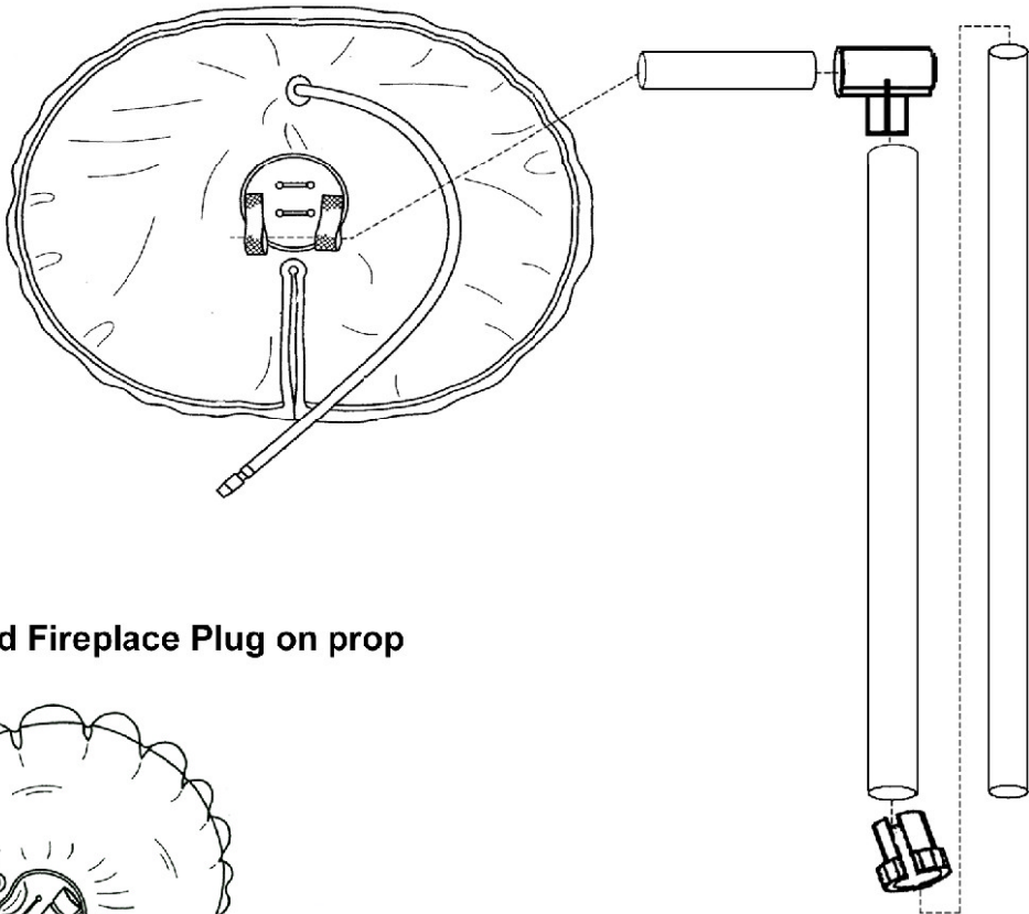
Fig 1: Assemble prop and Fireplace Plug as shown
